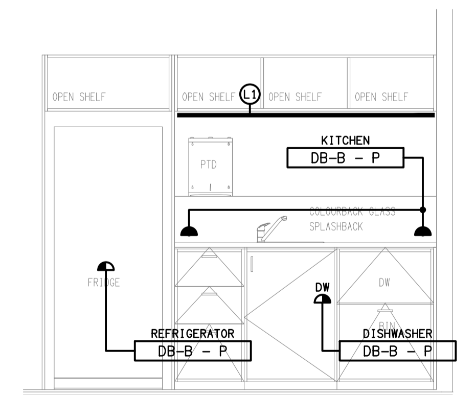
DETAIL A BOARD ROOM KITCHENETTE ELEVATION SCALE 1: 25
